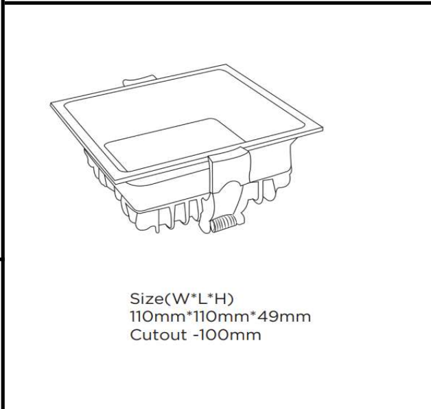
Dimension diagram
